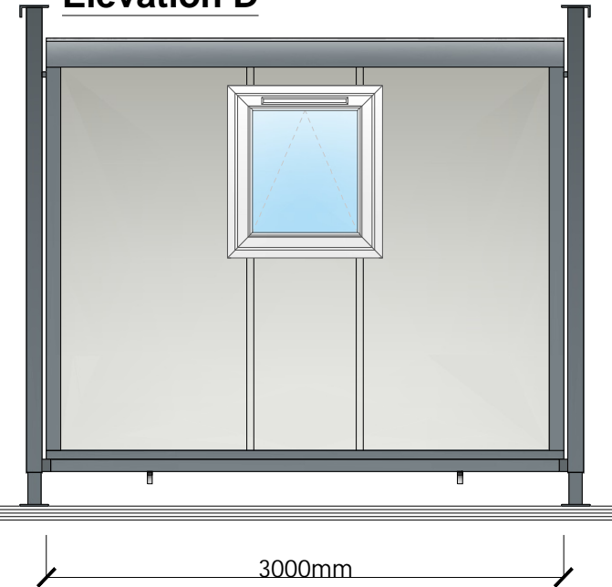
Elevation D
