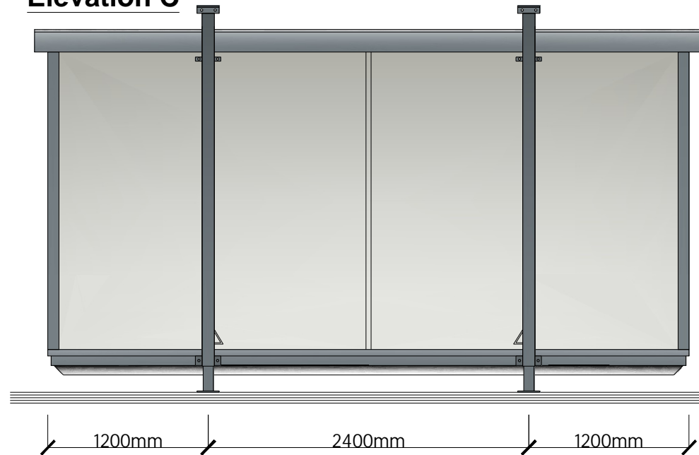
Elevation C
